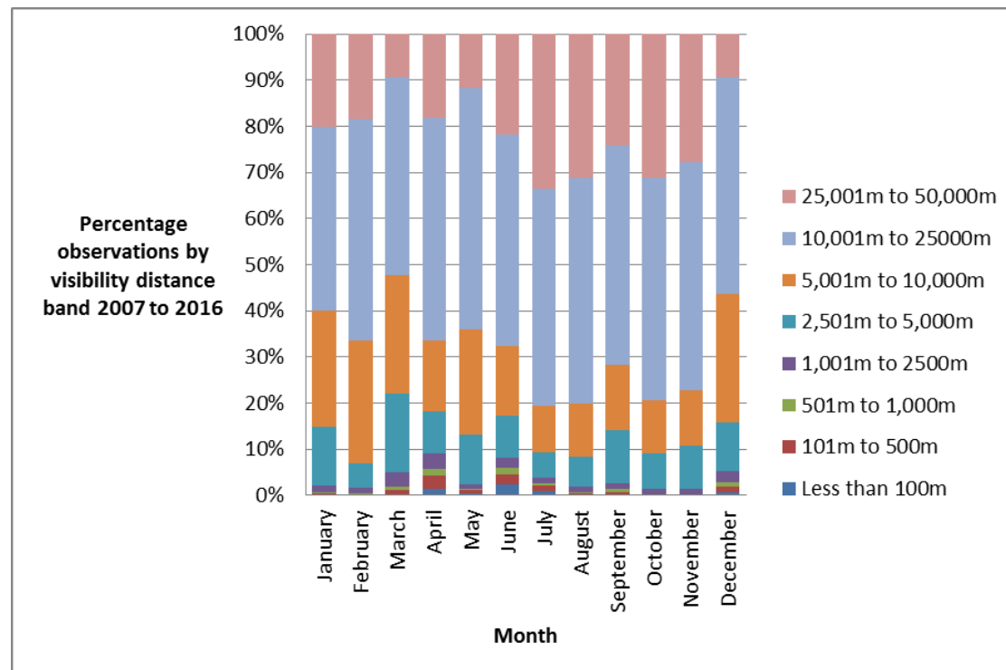
Figure 4.7: Monthly Met Office visibility data for the period 2007 to 2016.
