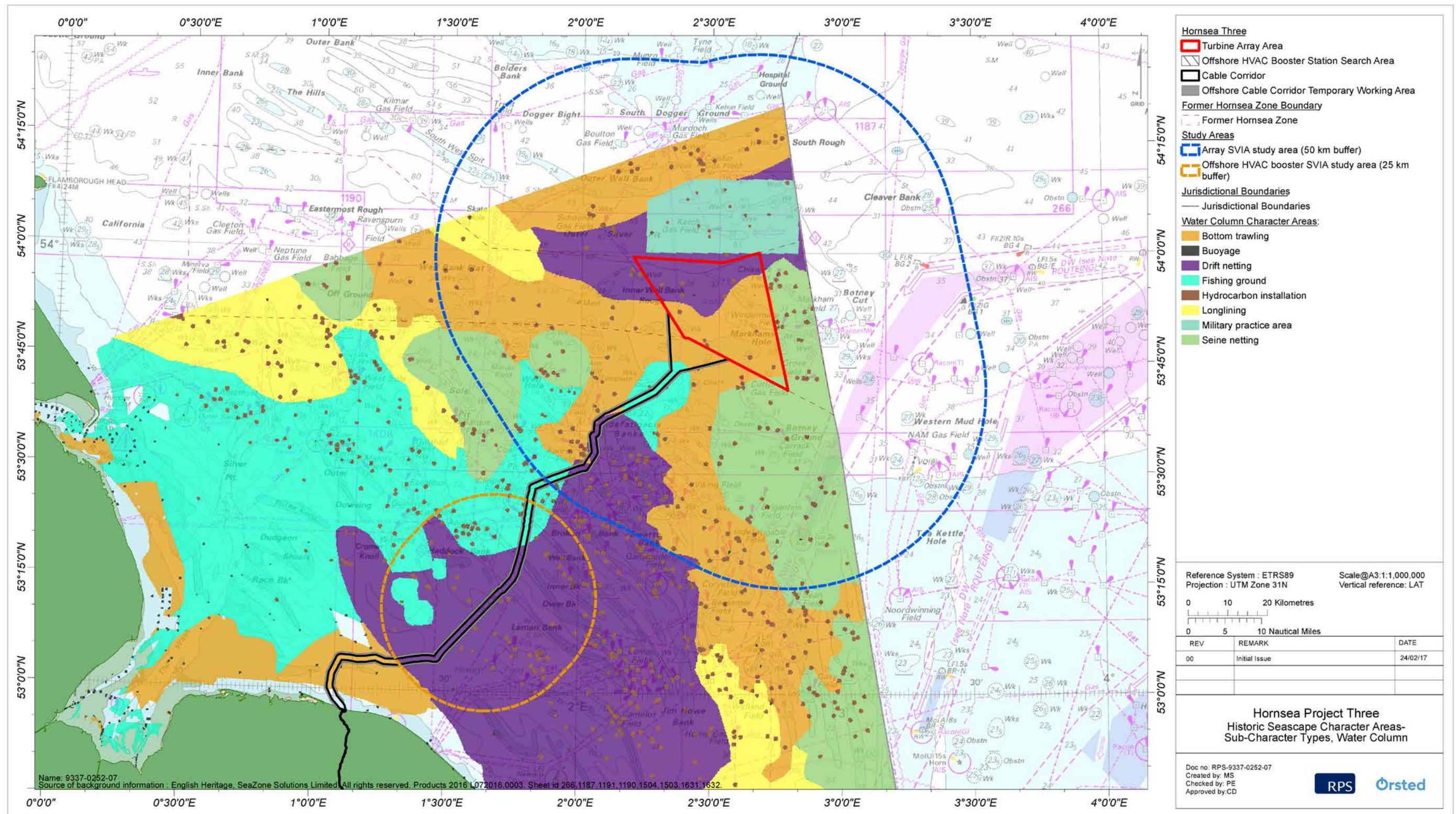
Figure 4.4: Historic Seascape Character SubTypes, Water Column, with Hornsea Three.
