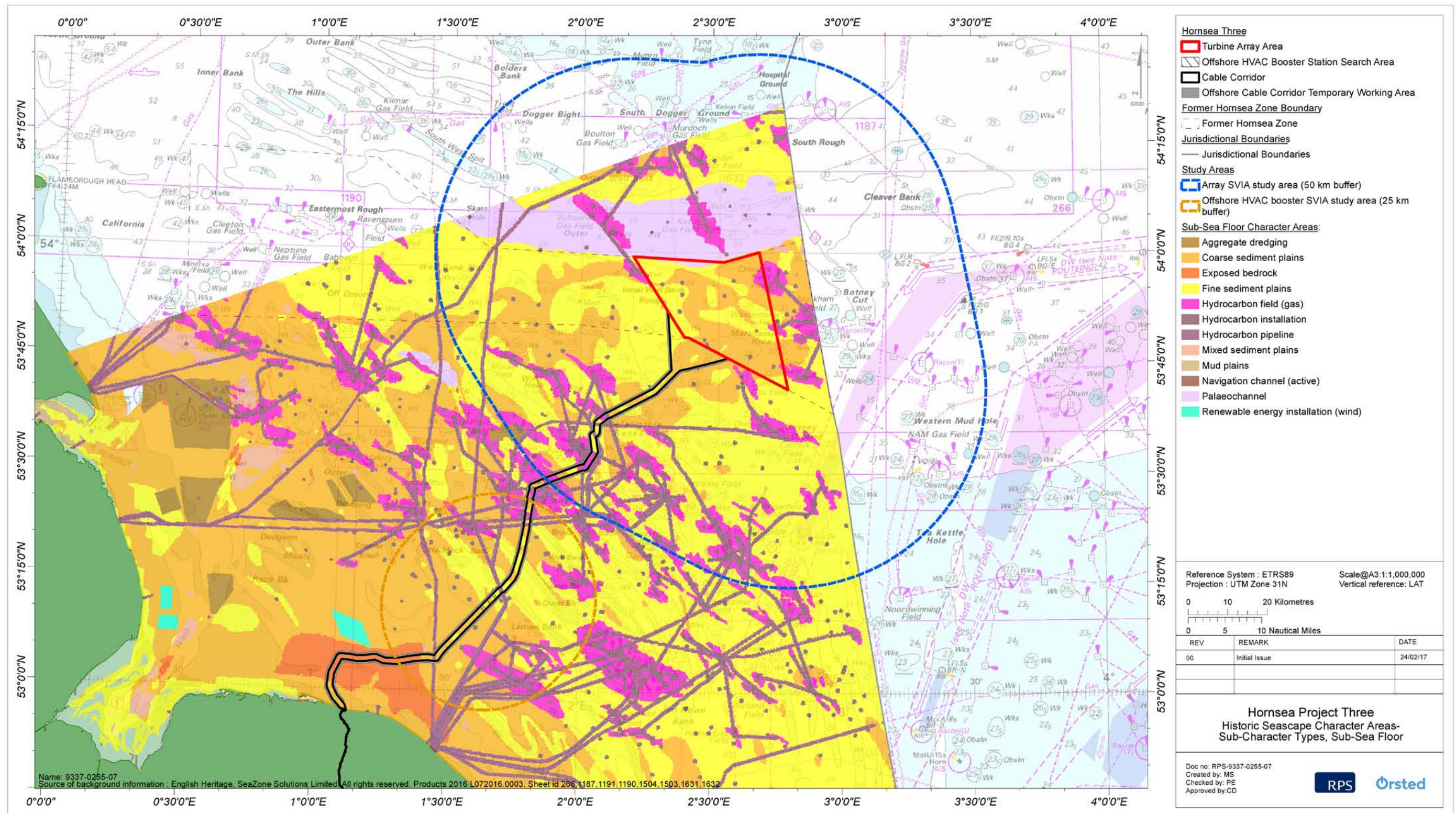
Figure 4.6: Historic Seascape Character SubTypes, Sub-Sea Floor, with Hornsea Three.
