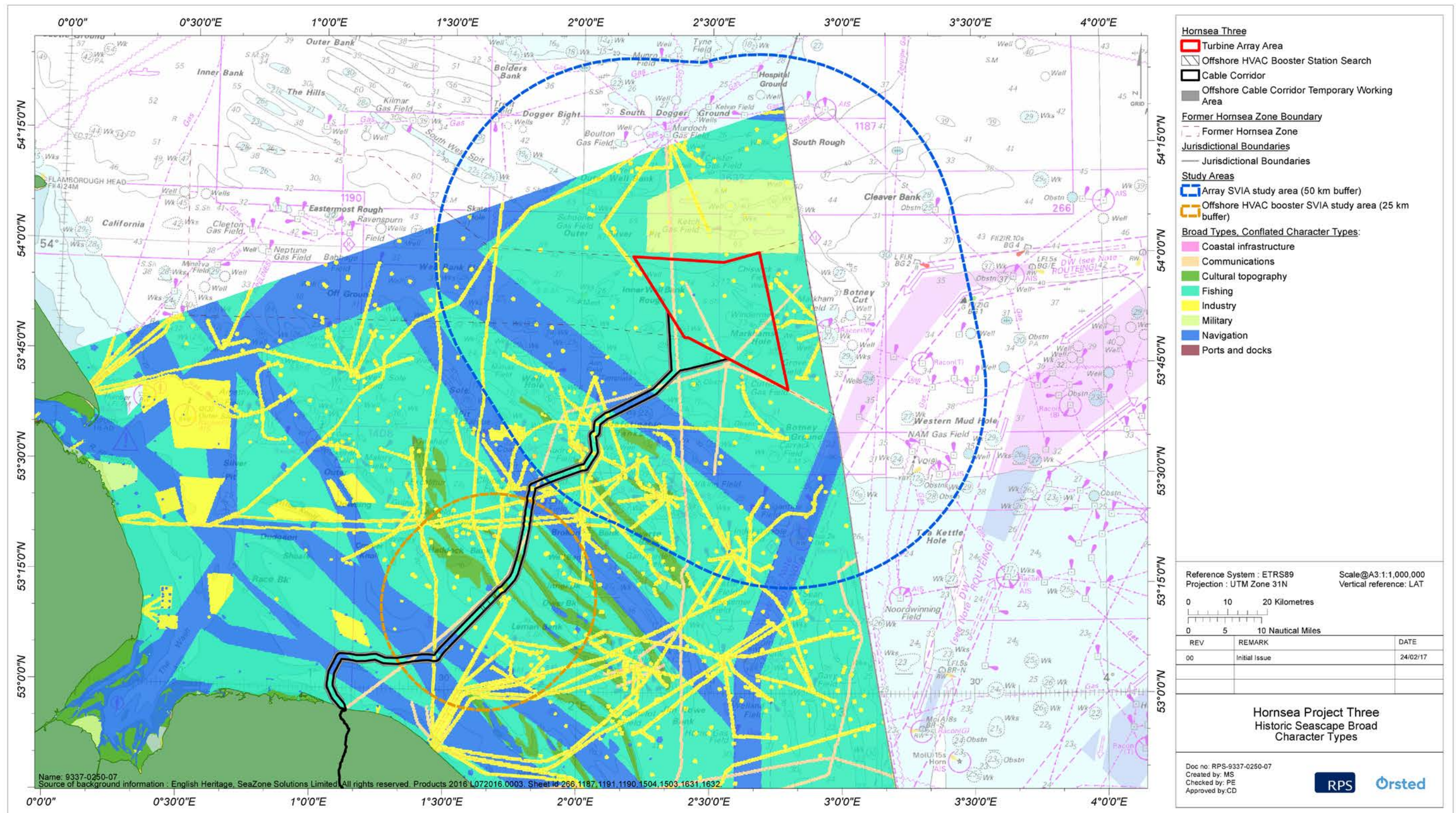
Figure 4.2: Historic Seascape Character Broad Types, Conflated, with Hornsea Three.
