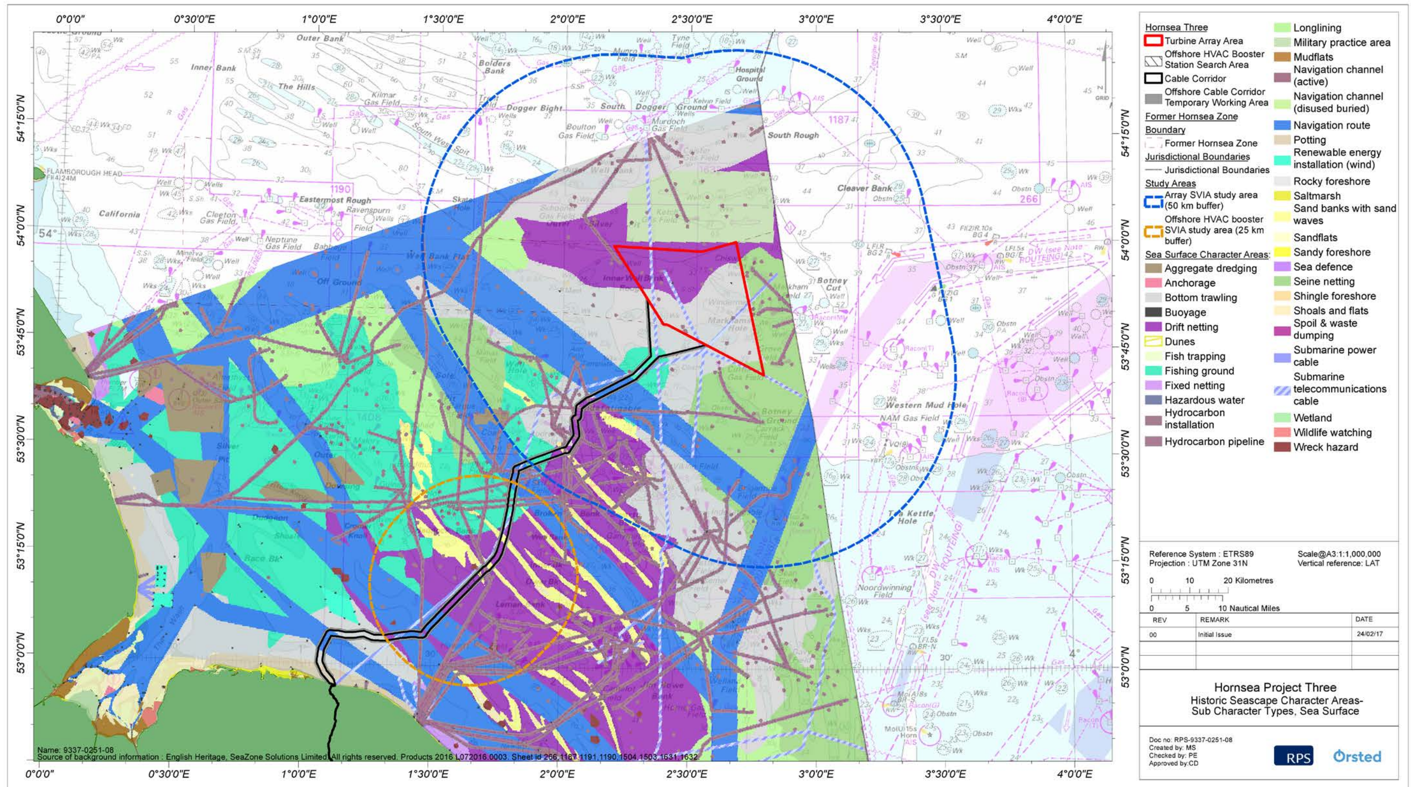
Figure 4.3: Historic Seascape Character SubTypes, Sea Surface, with Hornsea Three.
