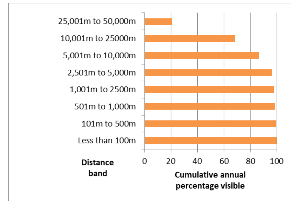
Figure 4.8: Cumulative percentage of visibility observations by distance band.
