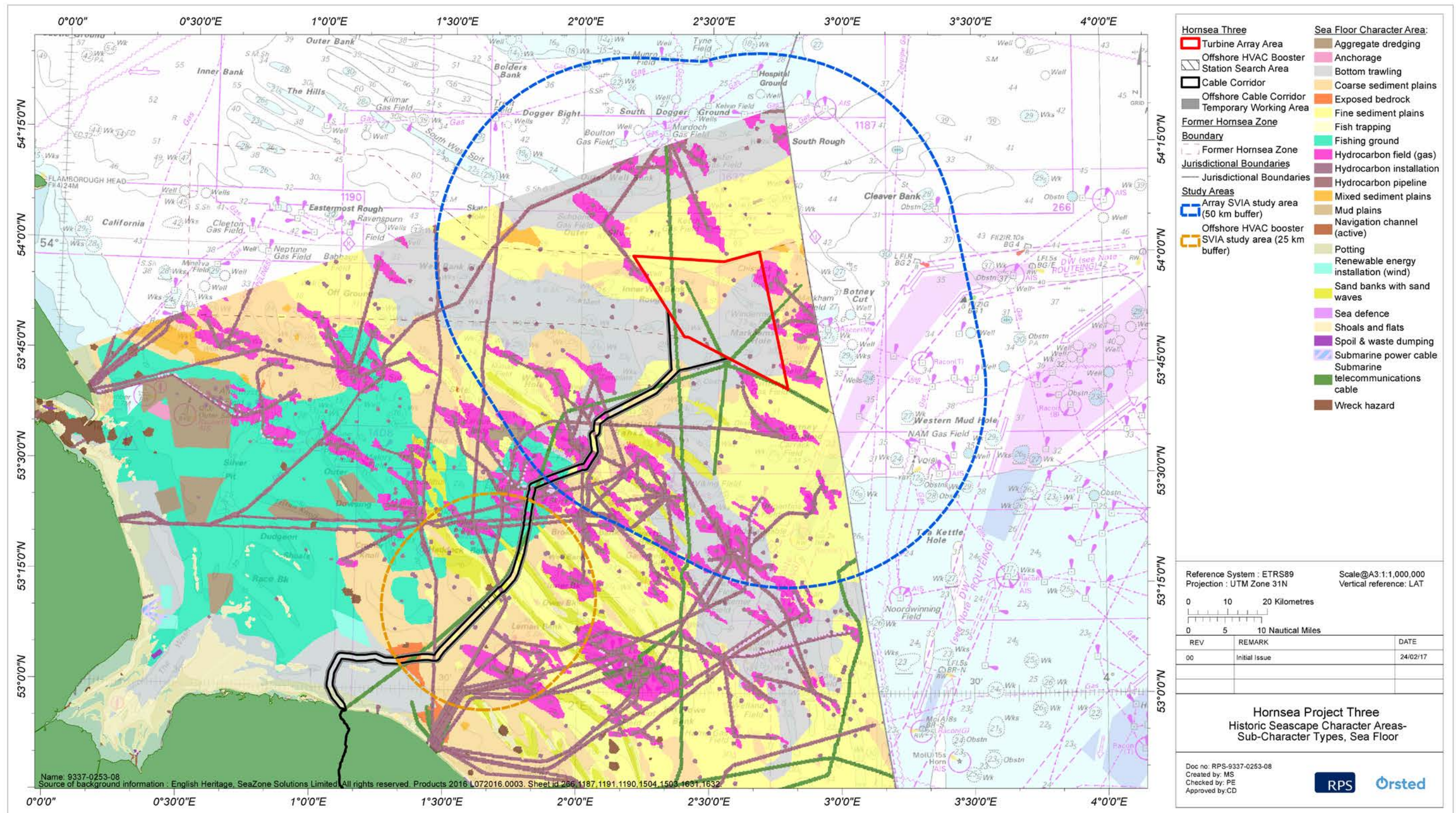
Figure 4.5: Historic Seascape Character SubTypes, Sea Floor, with Hornsea Three.
