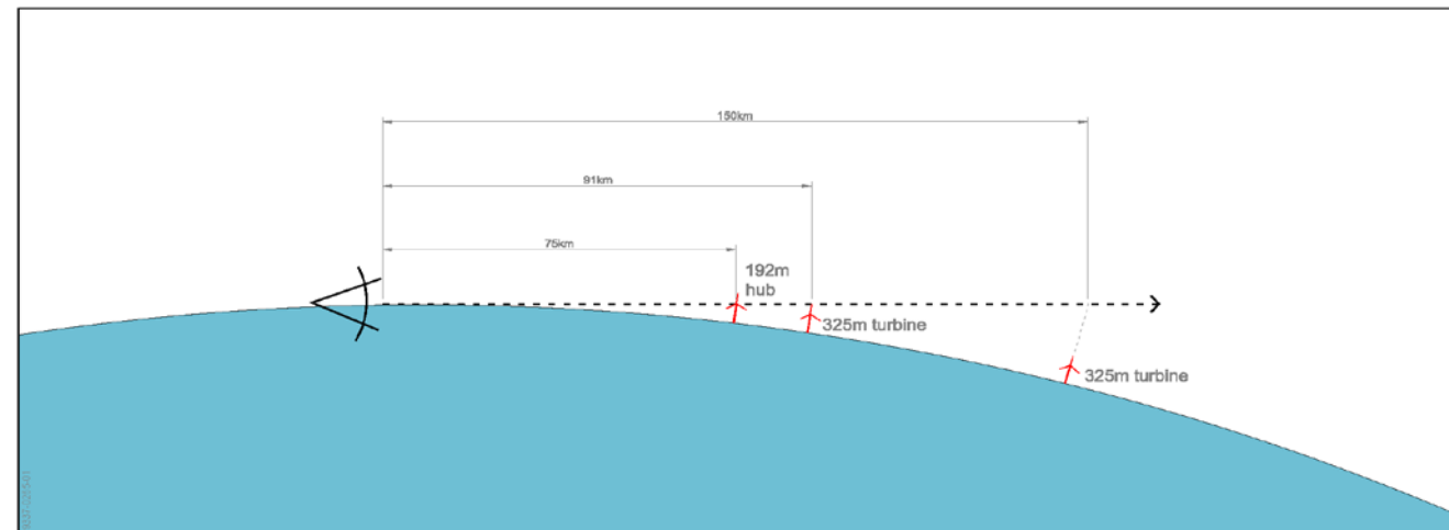
Figure 4.9: Illustration of the effects of curvature of the earth on visibility (not to scale).
